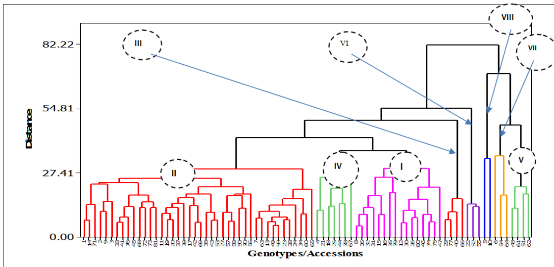
Fig. 1. Cluster groups of 81 coriander genotypes based on 21 different traits at Adami Tulu Agricultural Research Center, 2011
