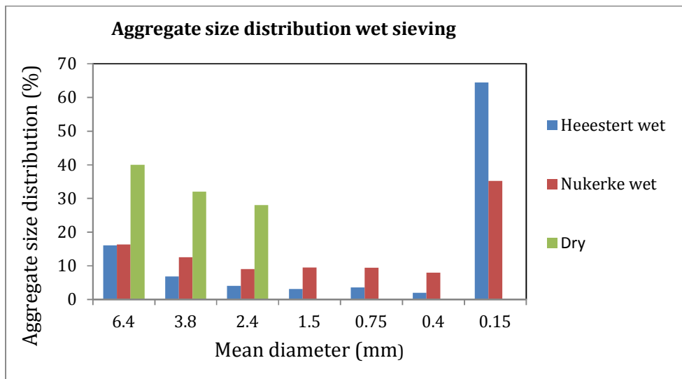
Fig. 2. Aggregate distribution (wet sieving) of soil samples
