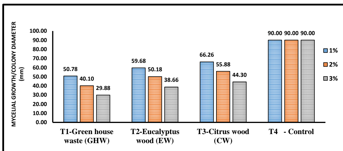
Fig. 1. Evaluation of bio-efficacy of different biochar's against Fusarium oxysporum f.sp. radicis-cucumerinum in In vitro condition
