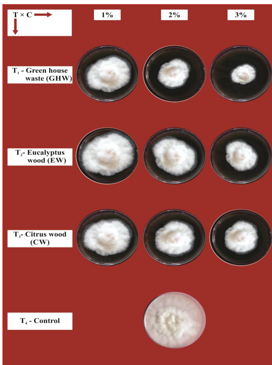
Plate 1. In vitro efficacy of different biochar's against Fusarium oxysporum f.sp. radicum-cucumerinum
