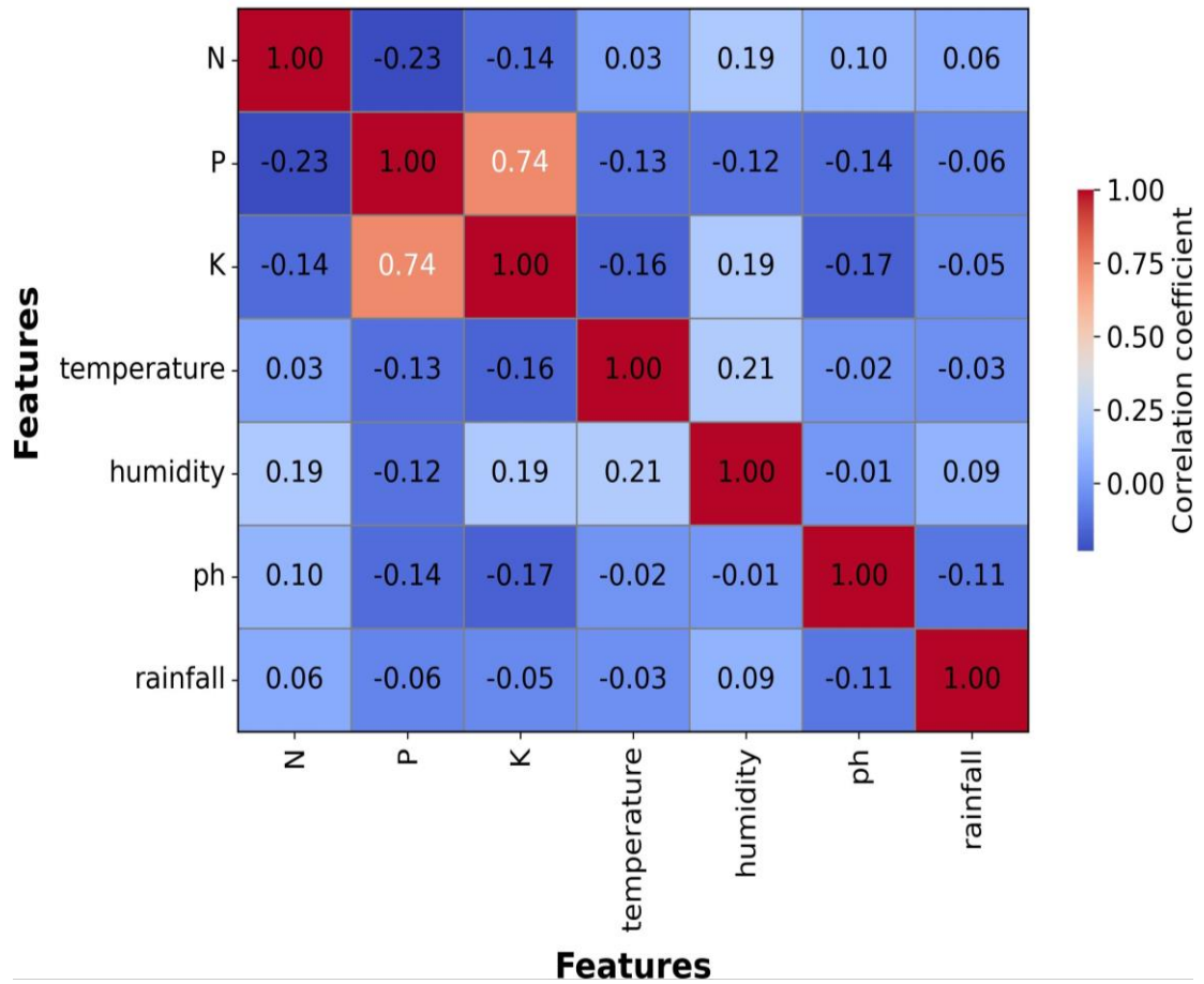
Fig. 4. Correlation Between Different Features
