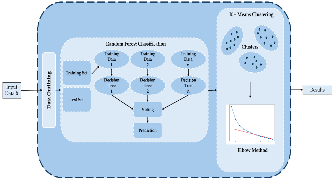
Fig. 2. Architecture of the Proposed Model
