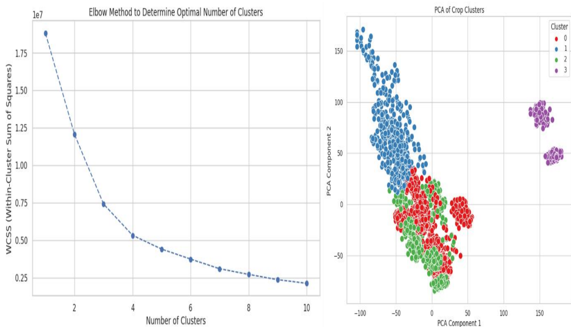
Fig. 5. Performance of K-means Clustering Analysis
