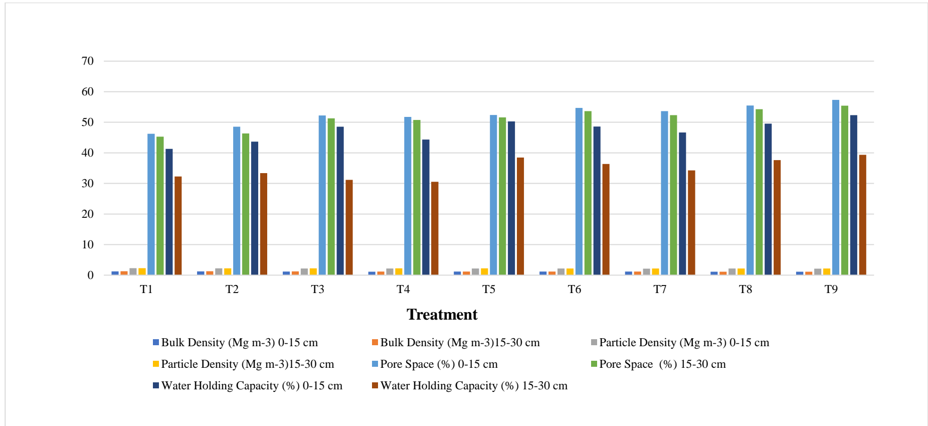
Fig. 1. Physical properties of soil sample after harvesting of cowpea
