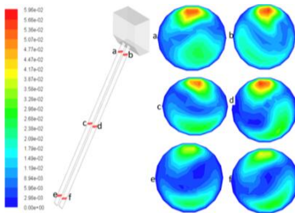
Fig. 11. Velocity contours at different axial positions in the tubes
