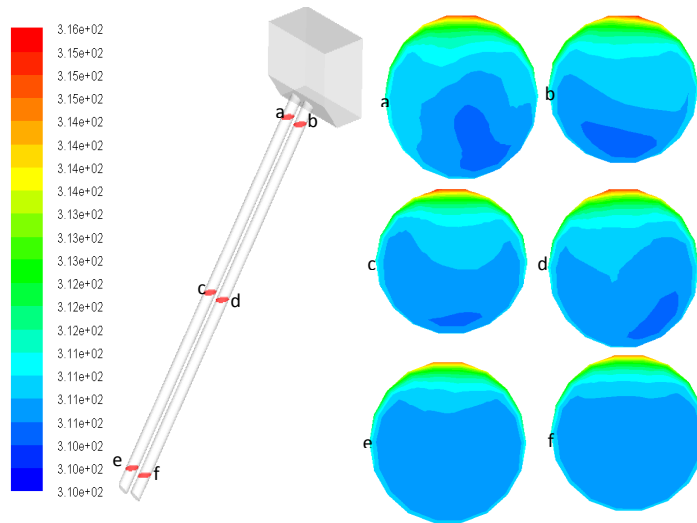
Fig. 10. Temperature contours at different axial positions in the tubes
