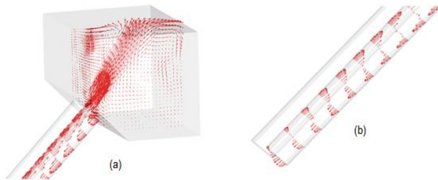
Fig. 9. Velocity vectors: (a) tank (b) tube
