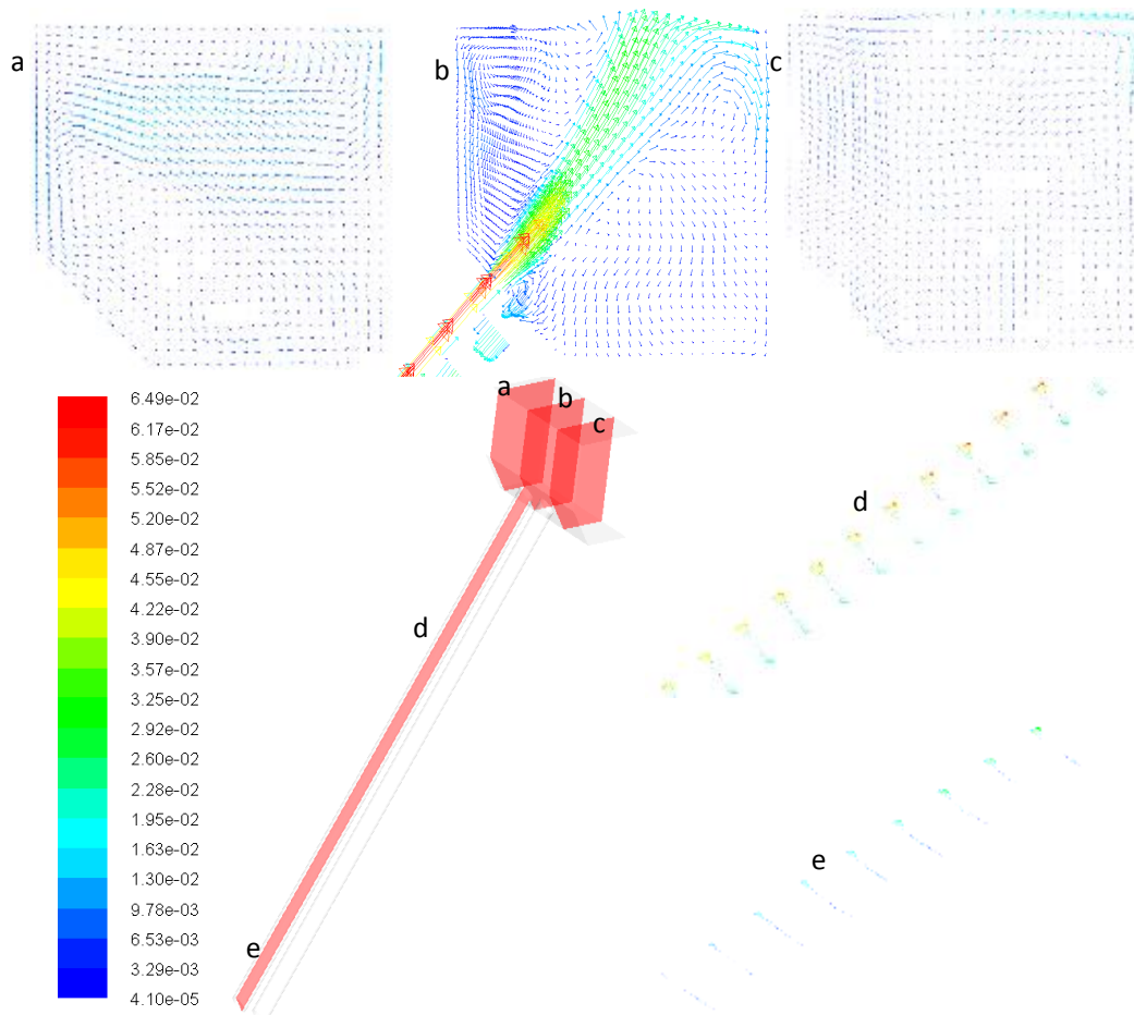
Fig. 13. Flow structure inside the system: (a, b, c) different positions inside the tank; (d) tube
