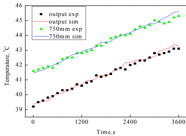
Fig. 12. Comparison: Measured and calculated temperature at two points
