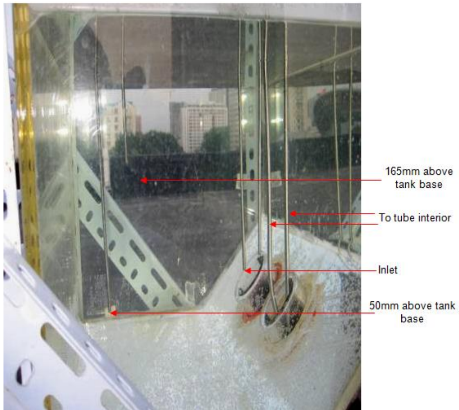
Fig. 3. Temperature measuring points
