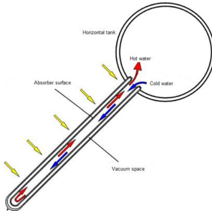
Fig. 1. Natural circulation in water-in glass solar water heater [7]
