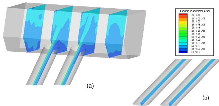
Fig. 8. Temperature distribution: (a) Main part of the system; (b) Near tubes closed end
