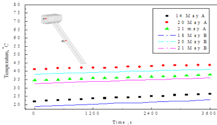
Fig. 7. Temperature comparison: Points inside the solar water heater for the three days
