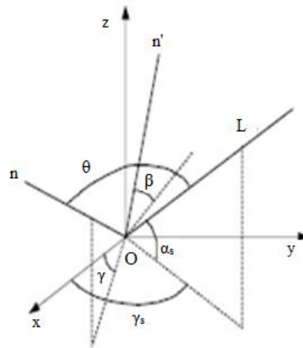
Fig. 5. The coordinate system for calculating incident angle Wei et al. [15]
