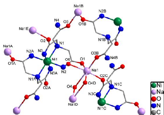
Fig. 1. Coordination environment around the Ni (II) and Na (I) ion in the complex at 30% probability thermal ellipsoids
