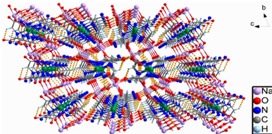
Fig. 2. Packing diagram of [\text{NiNa}_2(\text{L})_2(\text{H}_2\text{O})_4]_n in the crystal viewed along the a-axis
