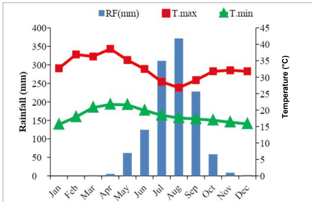
Fig. 2. Mean monthly rainfall (mm), maximum and minimum temperature (°C) (2012-2016) Source: Tigray meteorological services center, 2017
