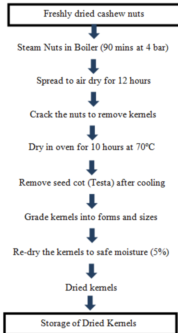
Fig. 1. Flow chart for processing raw cashew nut into kernels
